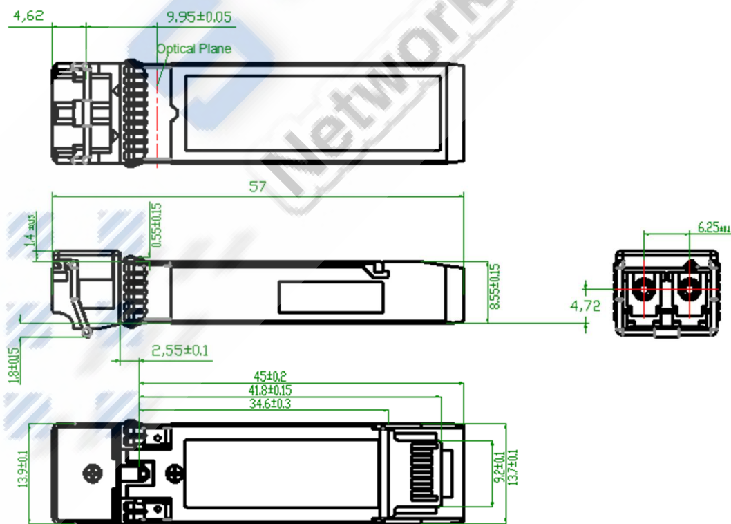
Figure 4 Mechanics drawing
