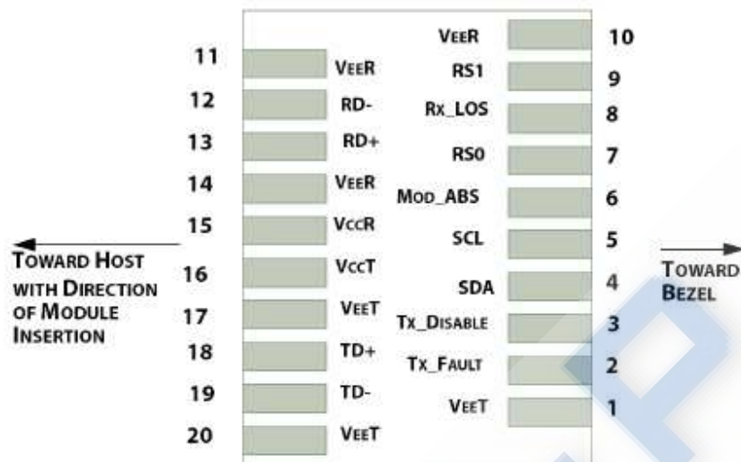
Figure 3, Pin View
