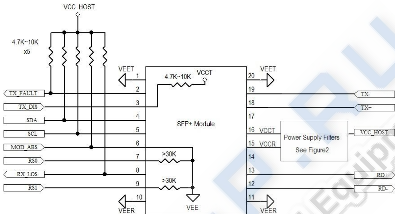
Figure4. Host-Module Interface
