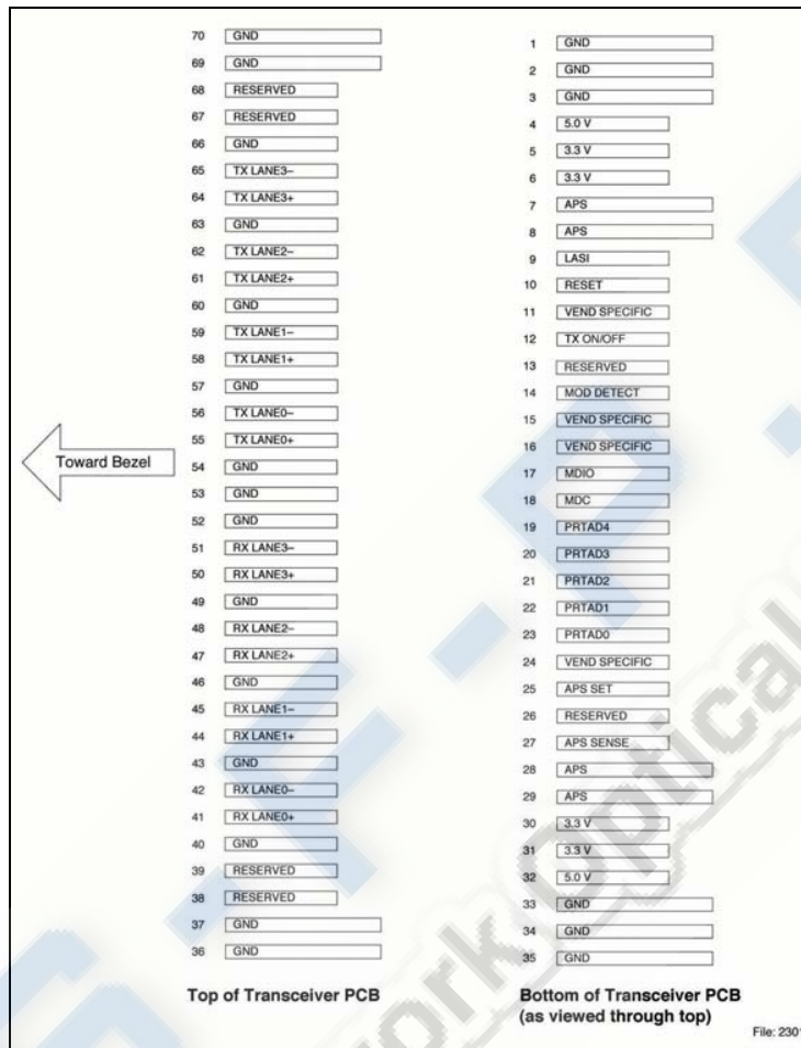
Fig 1-X2 Transponder Electrical Pad Layout
