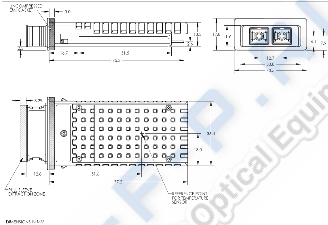
Figure 2-X2 Mechanical Dimensions
