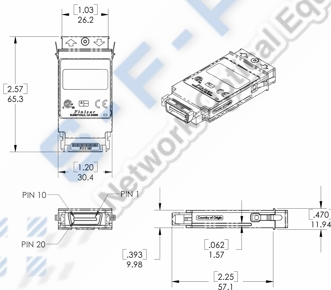
Figure 1. FTL-1619-XX Outline Drawing
