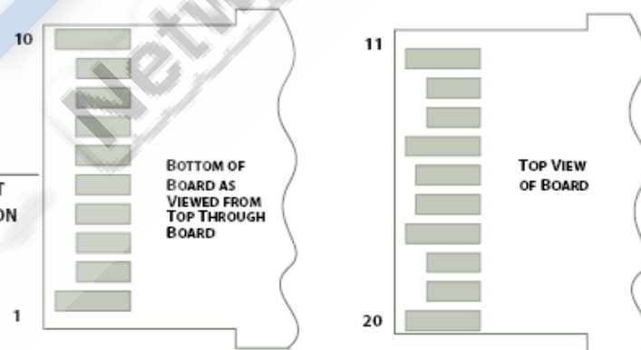
SFP+ module contact assignment
