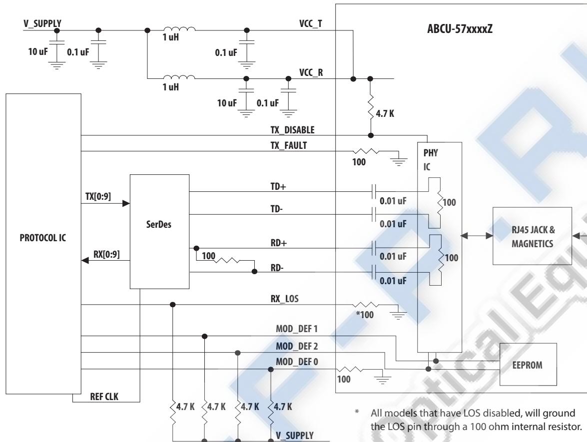
Figure 4. Typical Application Configuration for ABCU-57xxxxZ
