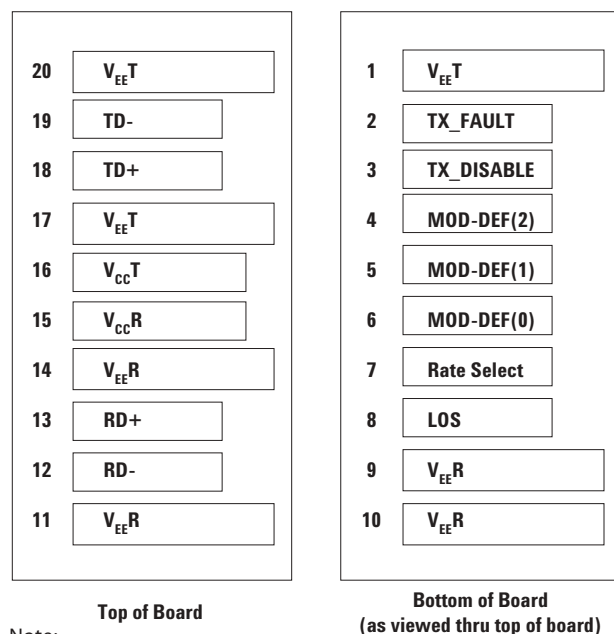
Note: TxFault , LOS and Rate_Select not used. Figure 2. 20-pin Connection Diagram of Module Printed Circuit Board
