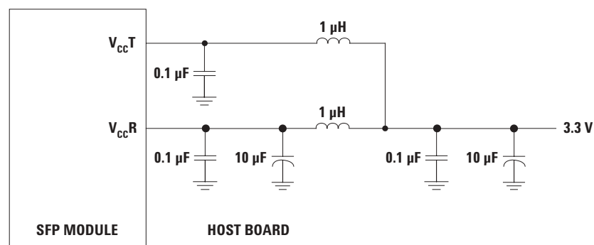
Note: Inductors must have less than 1ohm series resistance per MSA Figure 5. MSA Recommended Power Supply Filter
