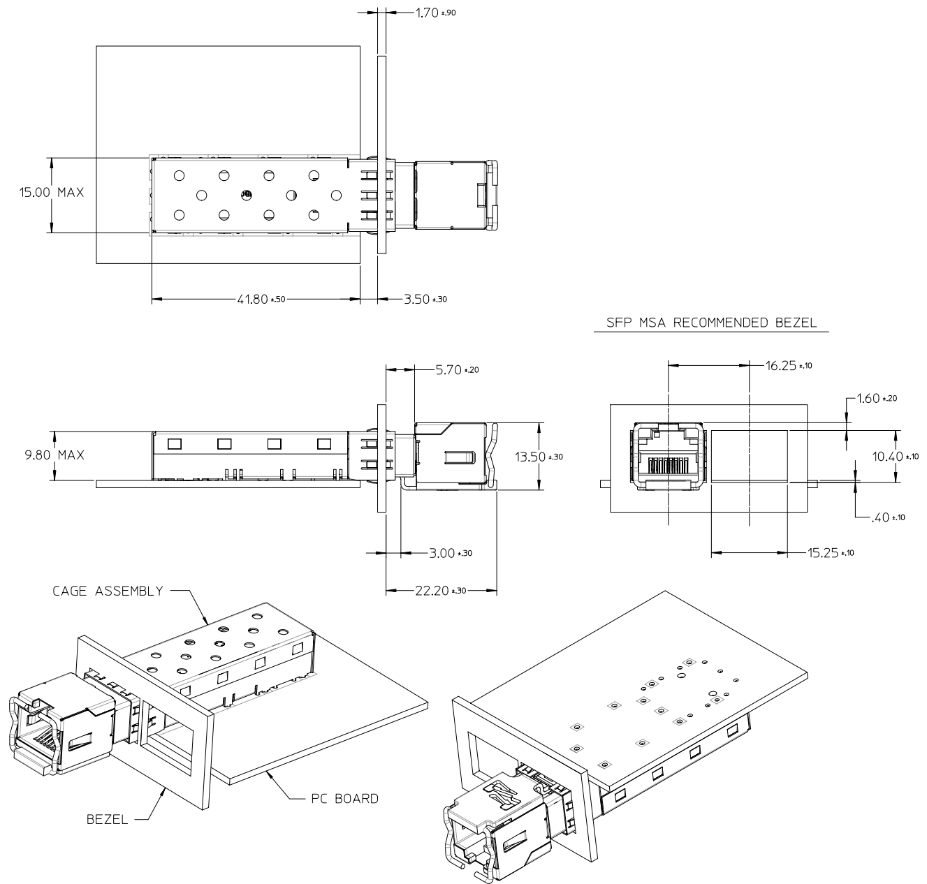
Figure 7b. Assembly Drawing
