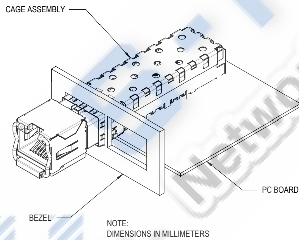
Figure 7b. Assembly Drawing
